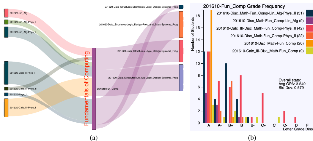
Figure 6. (a): the cropped view of the Sankey diagram showing the funnel course Fundamentals of Computing and various filters with grouping students by term courses. All grade levels and courses are selected. The cutoff is enabled. Groups are sorted by GPA, and the range for both group and link is set to [5, 200]. (b): the histogram of term-course groups GPA for the funnel course.
