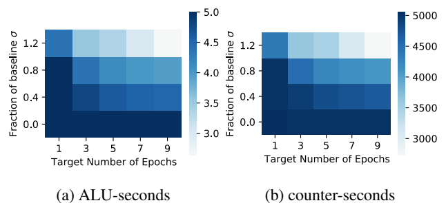
Figure 9: Evaluation of median resource usages for selected accuracy (y-axis) and latency (x-axis) targets for a single query. Lighter colors indicate lower resource usages.
