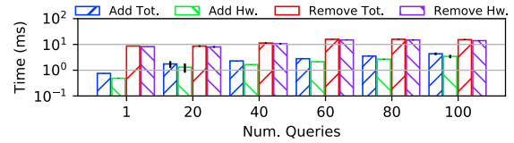
Figure 12: Hardware overheads as function of number of queries.
