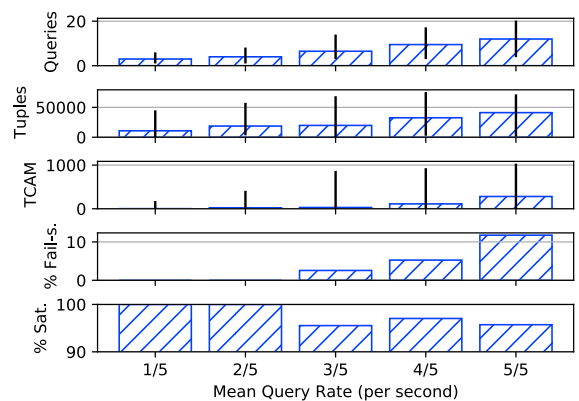
Figure 8: Performance of DynATOS on dynamic query workloads.
