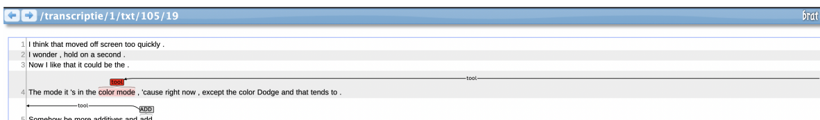
Figure 5: Annotation Tool
