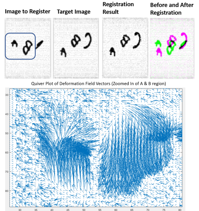
Figure 5: Pixel level Registration of two different MNIST letter projections and corresponding deformation field for a region.
