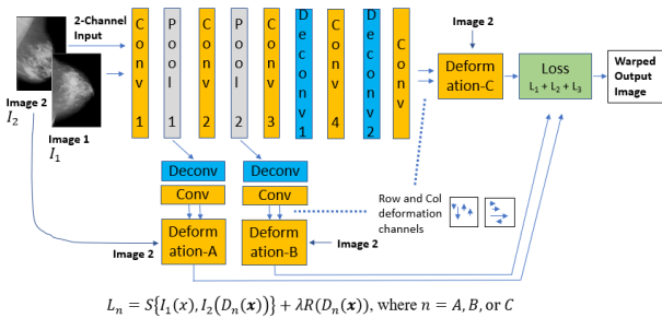
Figure 1: Pixel Level Registration CNN Architecture.
