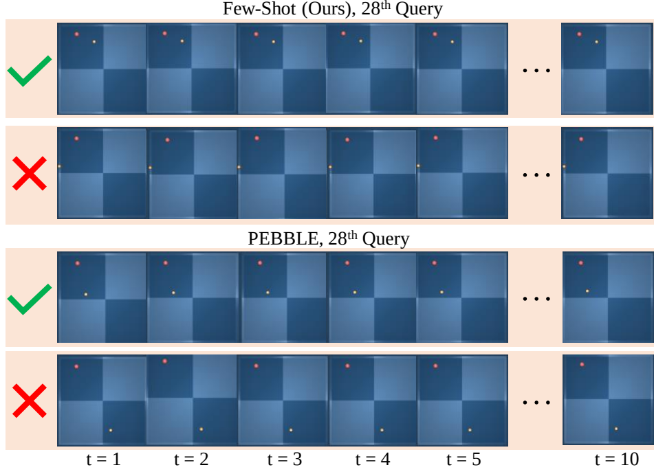
Figure 15: A depiction of the 28th query asked to users when training the Point Mass Agent from human feedback. The winning query was chosen based on proximity of the agent (yellow) to the goal position (red). At this point in training, our Few-Shot method sampled queries closer to the goal position than PEBBLE.
