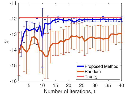
(a) \delta = 1
