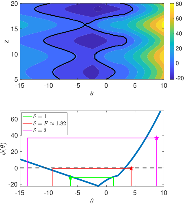
Figure 1: (Top) Contour plot for the KS function. The black line representing a value of 0. (Bottom) The minimum KS aggregated constraint violation value for every \theta , which is given by (15). Three different boxes are shown for three different \delta values, with the value of \theta that leads to the worst-case violation shown with a star.
