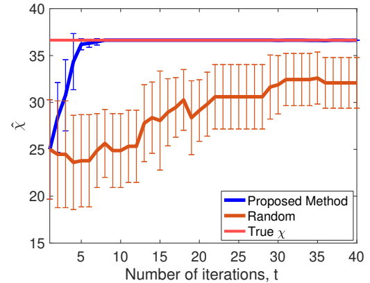
(b) \delta = 3
