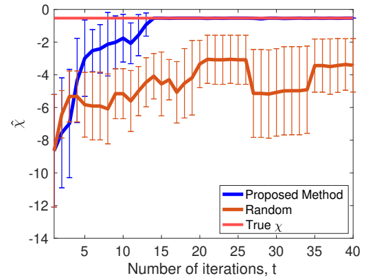
(c) \delta = 1.8125
