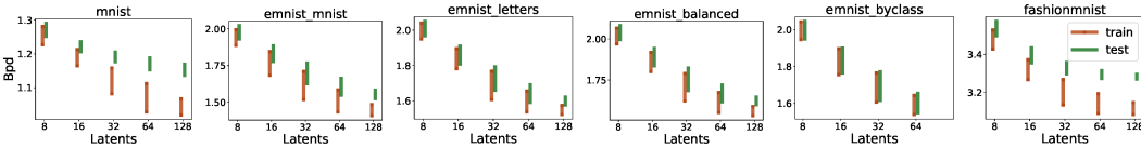
Figure 9: Structure learning via 75% pruning, growing and finetuning. We report bpd (y-axis) on both train (red) and test set (green) in terms of the number of latent states (x-axis). For each curve, training starts from the top (large bpd) and ends at the bottom (small bpd).
