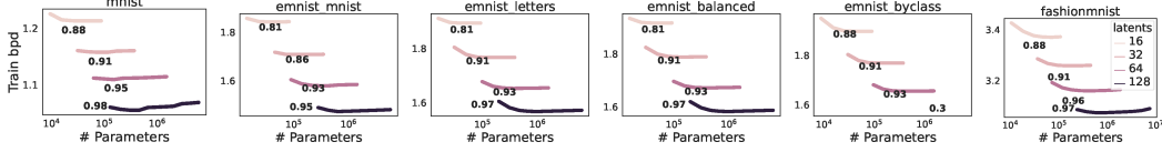
Figure 8: Model compression via pruning and finetuning. We report the training set bpd (y-axis) in terms of the number of parameters (x-axis) for different numbers of latent states. For each curve, compression starts from the right (initial PC |\mathcal{C}^{\text{init}}| ) and ends at the left (compressed PC |\mathcal{C}^{\text{com}}| ); compression rate (1 - |\mathcal{C}^{\text{com}}| / |\mathcal{C}^{\text{init}}|) is annotated next to each curve.
