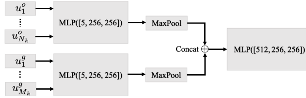
Figure 4: Architecture for the set feasibility predictor
