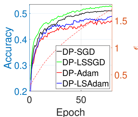
Figure 6: Performance comparison between different differentially private optimization algorithms in training CNN for CIFAR10 classification with a fixed \delta = 10^{-5} .
