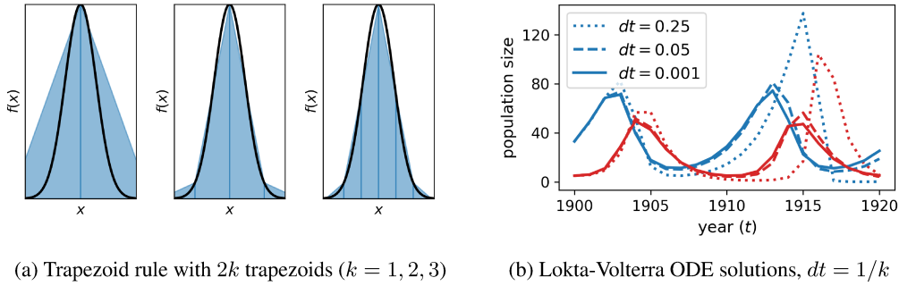
Figure 1: Examples of low-fidelity sequences of models. (a) Sequence trapezoid quadrature estimates I_k , where I_k is the trapezoid rule with 2k trapezoids. (b) Lotka-Volterra ODE solutions for prey u(t) (blue) and predator v(t) (red) using Euler’s method with step size dt .
