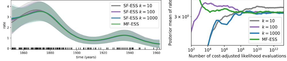
Figure 3: Coal mining disasters 1850–1963. Left: Posterior mean of the rate function at the observed data points. Right: Posterior mean of the rate function at T = 1862 vs computation.
