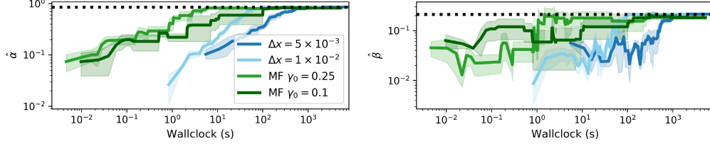
Figure 5: PDE-constrained optimization with a linear heat equation. Estimate for \alpha (left) and \beta (right) vs computation. The black dotted lines denote the true values of \alpha, \beta .
