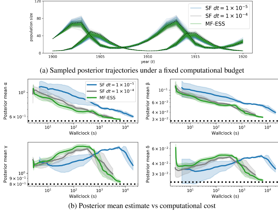
Figure 4: Lotka-Volterra system parameter identification. The fidelity represents (a function of) the step size dt of the ODE solver.
