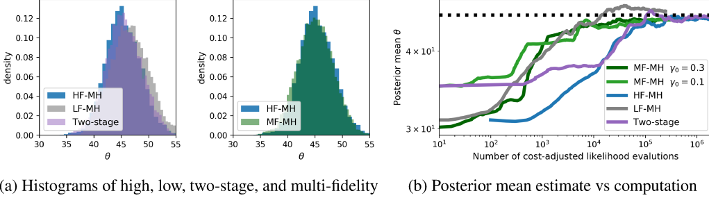
Figure 6: Parameter inference in a Gaussian process regression model. Left: The posterior distribution of the parameter \theta . Right: The posterior mean estimate vs computational cost.
