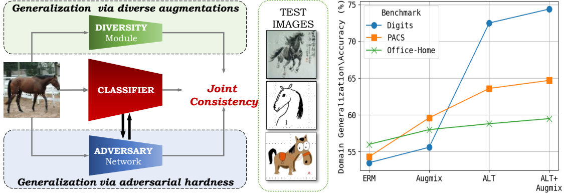
Figure 1. ALT consists of a diversity module (data augmentation functions such as Augmix [21] or RandConv [42] and an adversary network (to learn image transformations that fool the classifier). We show an example from the PACS benchmark under the single-source domain generalization setting, with real photos (P) as the source domain and art paintings (A), cartoons (C), and sketches (S) as the target domains. The plot summarizes our results – while diversity alone improves performance over the naive ERM baseline, adapting this diversity using adversarially learned transformations (ALT) provides a significant boost for domain generalization on multiple benchmarks.
