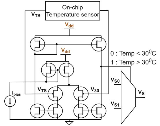
Fig. 5: Multiplexing sensor output for reliable operation over a broad temperature range. During an attack, both inputs to the comparator experience similar voltage modulation and select the appropriate sensor for detection.
