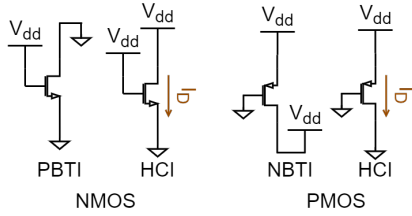
Fig. 4: Aging conditions in NMOS and PMOS.
