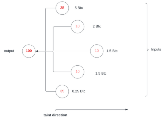
Figure 1: HOLO, which is a combination of TIHO and LIFO
