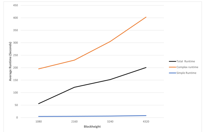
Figure 4: Average Runtime Across all Addresses
