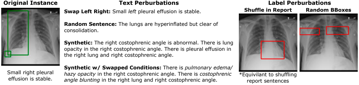
Figure 10: Examples of each perturbation (including Synth w/ Swapped Conditions ) for a given instance.
