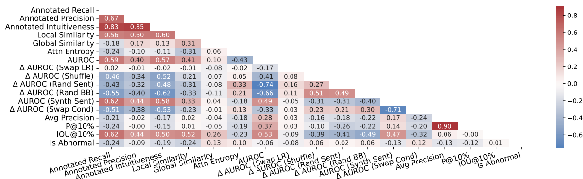
Figure 19: GLoRIA Retrained
