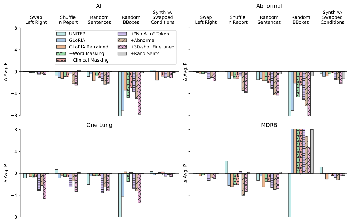
Figure 14: \Delta AUROC for all models and subsets.
