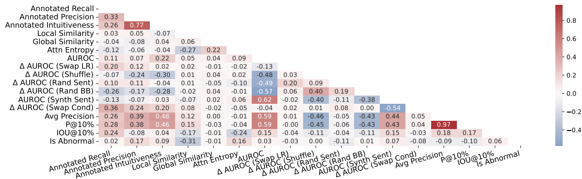
Figure 18: GLoRIA
