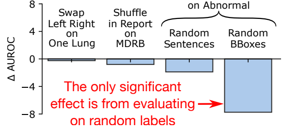
Figure 3: For each perturbation, we plot the change in localization performance (AUROC) of GLoRIA .
