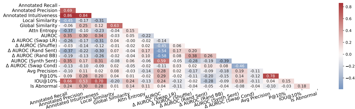
Figure 20: +Word Masking
