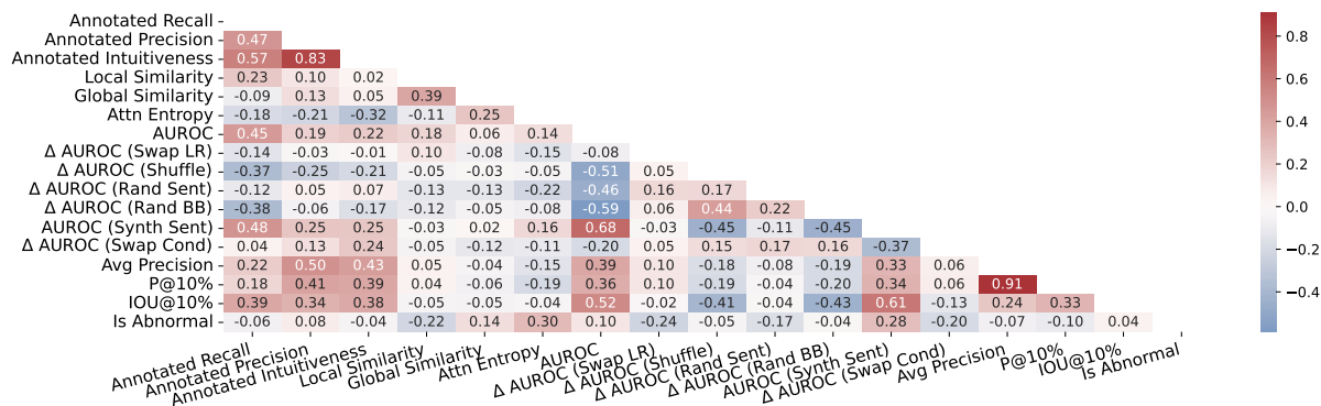
Figure 24: +30-shot Finetuned
