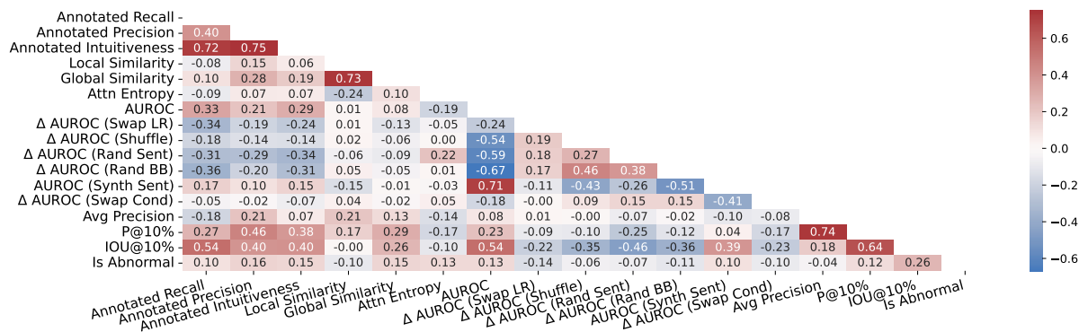
Figure 23: +Abnormal
