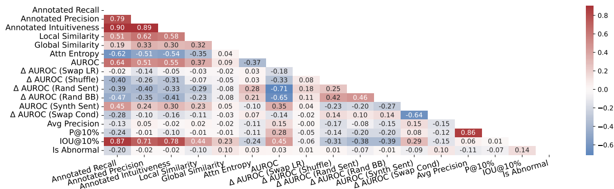
Figure 21: +Clinical Masking
