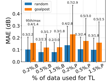
Fig. 3: MAE of EDFA gain prediction accuracy with varying target to source data size ratios ( N_{tgt}/N_{src} ) used for TL.
