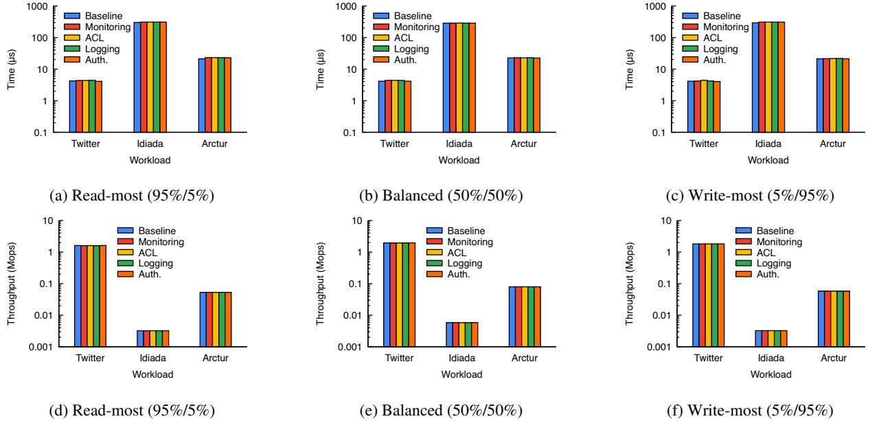
Figure 10: The request completion time and throughput under realistic workloads.
