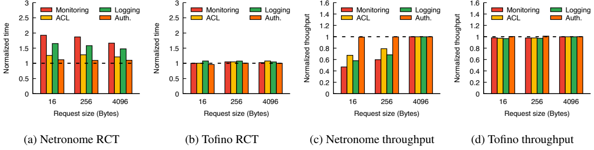
Figure 11: The request completion time (RCT) and throughput of Bedrock deployed in the Netronome NIC and Tofino switch. The number has been normalized to their baselines respectively.
