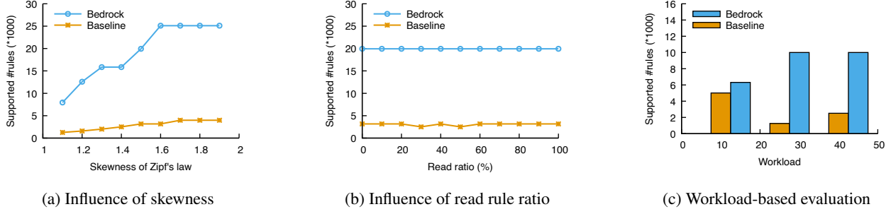
Figure 5: Bedrock outperforms the baseline by its ACL compression techniques. We further measure Bedrock under different skewness of memory region sizes, read/write rule ratios, and use realistic workloads based on Twitter, Idiada, and Arctur traces.
