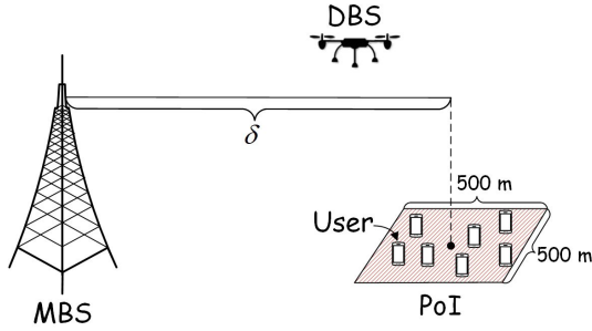
Fig. 3. Simulation setup.
