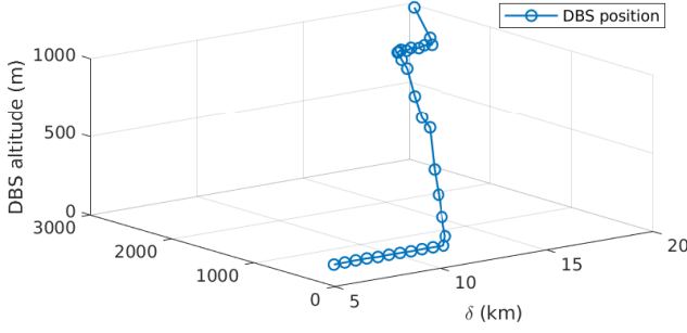
Fig. 5. DBS position over \delta .
