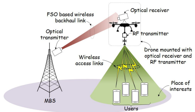
Fig. 1. FSO-based drone-assisted mobile network architecture.
