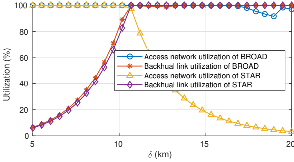
Fig. 6. Utilization over \delta .
