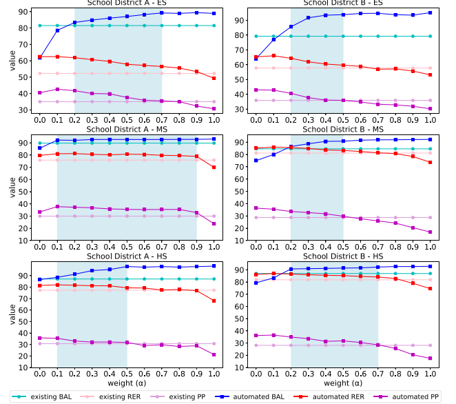
Figure 3: Study of different weight parameters.
