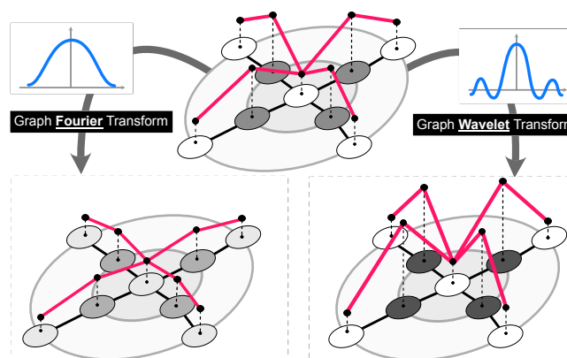
Figure 1: The graph Fourier transform smooths out an abrupt signal, whereas the graph wavelet transform accentuates it.
