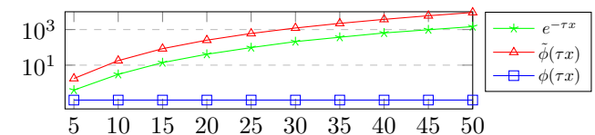
Figure 5: Ablation test of admissibility condition. X- and Y-axis denotes scale ( \tau ) and MSE.
