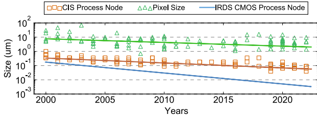
Fig. 3: CIS process node always lags behind conventional CMOS process node. This is because CIS node scaling tracks the pixel size scaling, which does not shrink aggressively due to the fundamental need of maintaining photon sensitivity.
