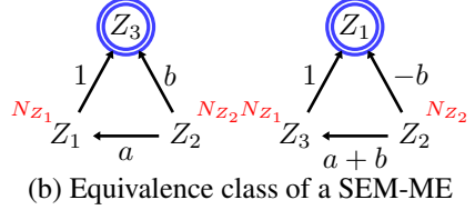
Figure 3: DOG Equivalence classes.
