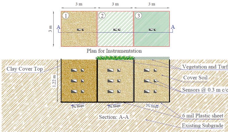
Fig. 2. Instrumentation plan and section.
