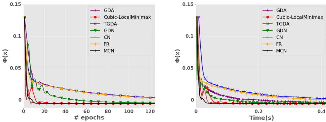
Figure 2: Comparison of all the algorithms for synthetic experiment.
