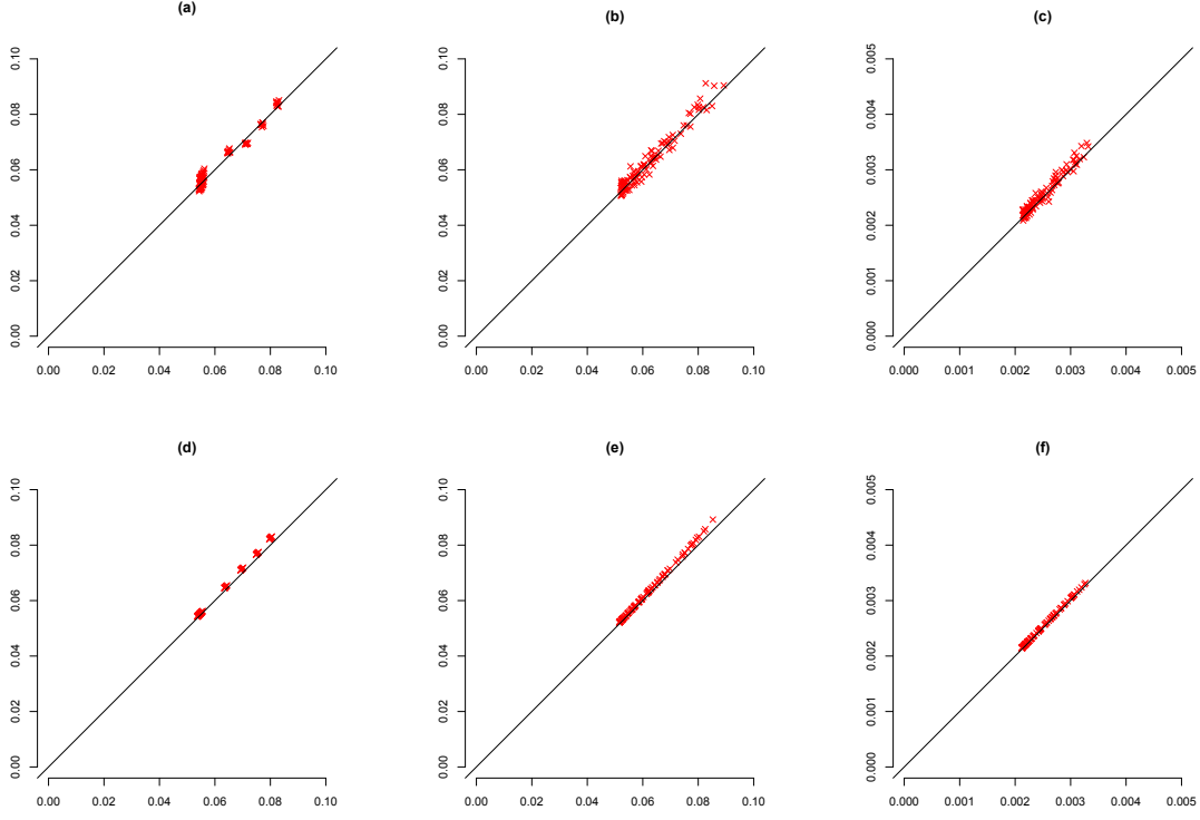
Figure 6: Panels (a)-(c) plot s^2(g) against \sigma^2(g) for g(M) = m_{ij} , \theta_i , and \beta_j , respectively, and Panels (d)-(f) plot s^2(g) against \tilde{\sigma}^2(g) for g(M) = m_{ij} , \theta_i and \beta_j , respectively, for the random design setting. Each panel shows 100 randomly sampled m_{ij} , \theta_i , or \beta_j under each setting. The line y = x is given as a reference.
