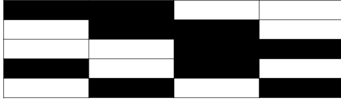
Figure 2: A heat map of Z . The black and white regions correspond to z_{ij} = 1 and 0, respectively.
