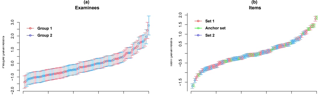
Figure 9: (a) 95% confidence intervals of 100 row parameters, with 50 randomly selected from each group. (b) 95% confidence intervals of the 100 column parameters, with 40 each randomly chosen from group 1 and group 2 and 20 randomly selected from anchor items (i.e., common items).
