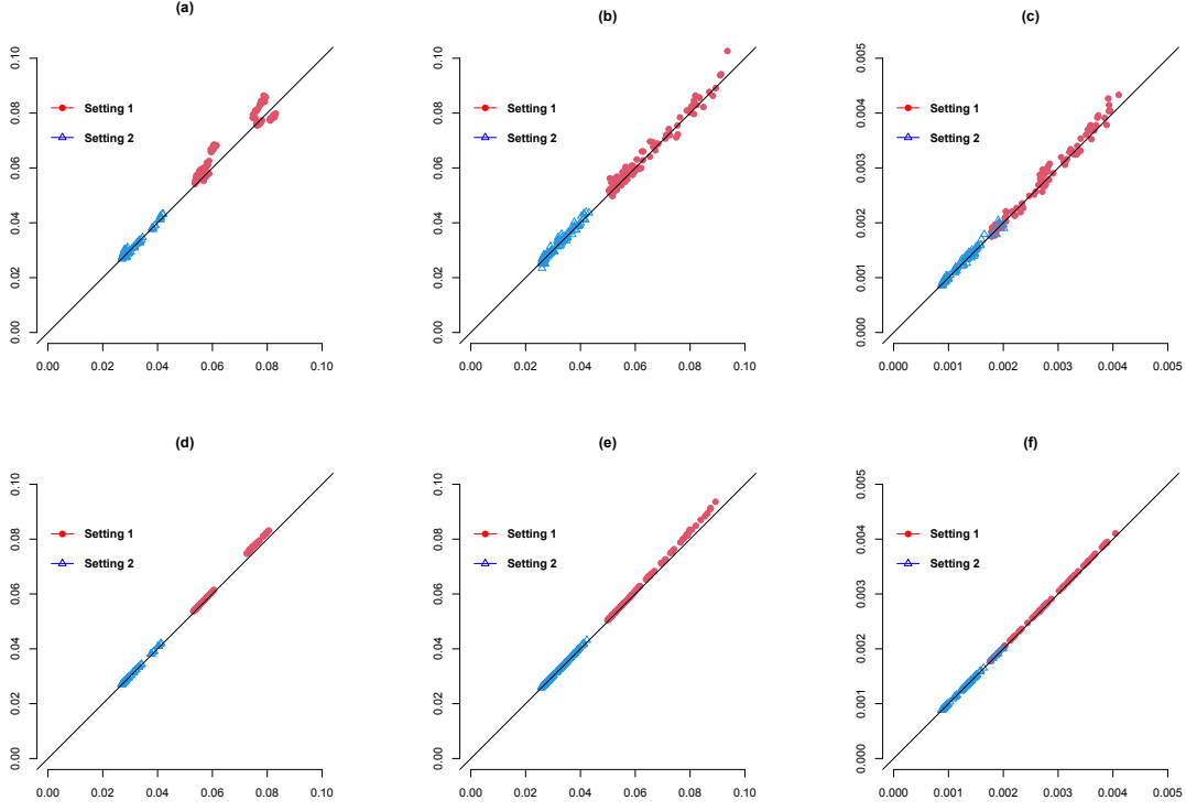
Figure 3: Panels (a)-(c) plot s^2(g) against \sigma^2(g) for g(M) = m_{ij} , \theta_i , and \beta_j , respectively, for fixed block-wise setting. Panels (d)-(f) plot s^2(g) against \sigma^2(g) for g(M) = m_{ij} , \theta_i and \beta_j , respectively, for fixed block-wise setting. Each panel shows 100 randomly sampled m_{ij} , \theta_i , or \beta_j under each setting. The line y = x is given as a reference.
