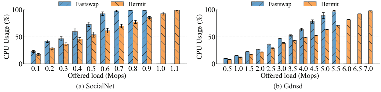
Figure 19: For SocialNet and Gdnstd, Hermit still saves 10%–40% CPU cycles under varying load compared with Fastswap, which is the key enabler it can achieve low tail latency under high load.
