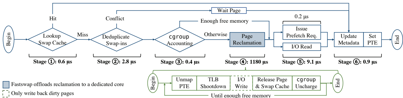
Figure 1: The life cycle of a remote memory page fault in Linux swap.
