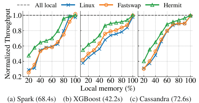
Figure 9: We measured the throughput of batch applications achieved by different swap systems normalized to the ideal local-only setup. Hermit outperforms other baselines. The number in the parenthesis shows the ideal execution time.
