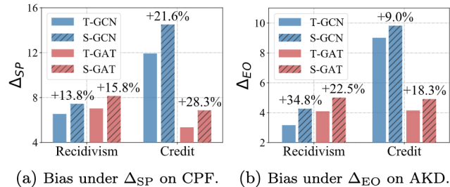
Figure 1: A comparison of exhibited bias between teacher and student models based on two representative GNN knowledge distillation frameworks (CPF and GraphAKD). "T" and "S" represent the teacher and the student model, respectively. The names of GNN mark out the corresponding teacher models.
