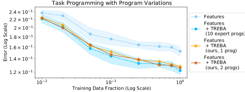
Figure 6: Applying symbolic encoders for self-supervision. “Features” is baseline w/o self-supervision. “TREBA” is a self-supervised approach in the Task Programming paradigm (Sun et al. 2021b), using either expert-crafted programs or our symbolic encoders as the weak-supervision rules. The shaded region is std dev over 9 repeats. The std dev for our approach (not shown) is comparable. Based on Sun et al. (2021b), the error is computed using 1.0 - \text{Mean Average Precision} .
