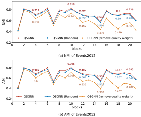
Figure 7: Results with different selection strategy and loss.
