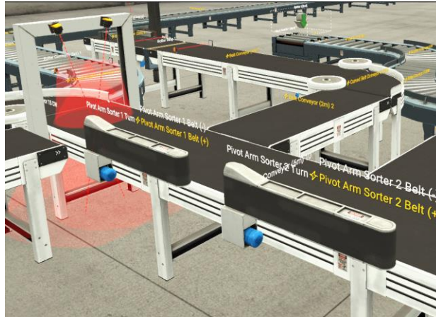
Figure 10: Color sensor gate
