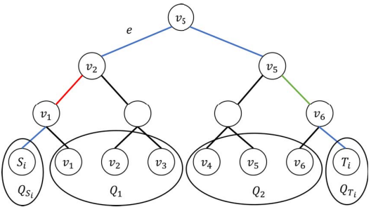
(b) A component-level path in blue. Red and green edges are crossing a component.
