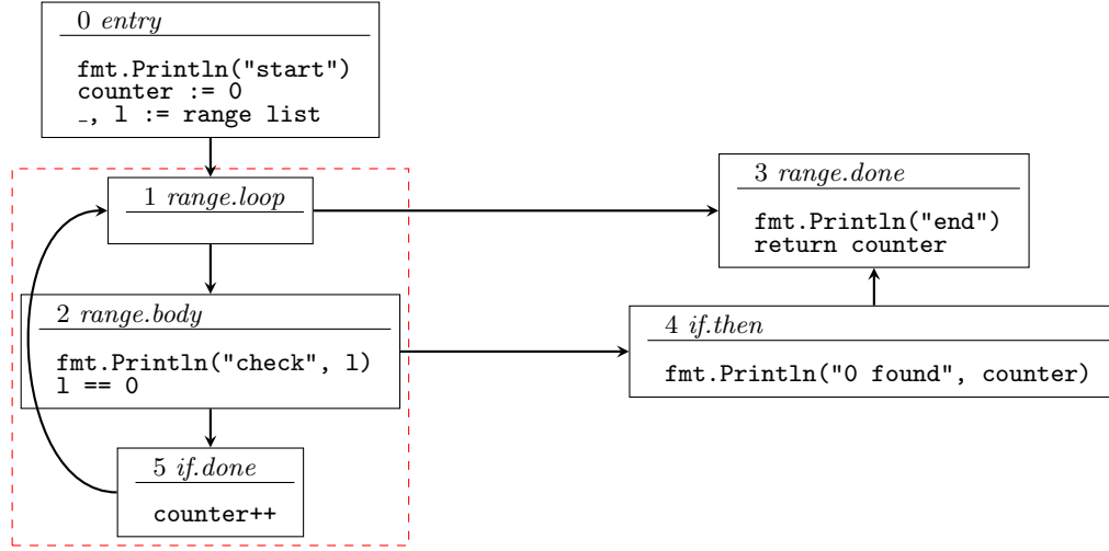
图 2 CFG of Listing 1 with a Red Dashed Frame of Strongly Connected Components
