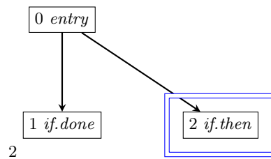
Figure 3 CFG of Listing 5 with a Blue Doubled Frame For the Block to be Reported (corresponding AST Nodes are abbreviated)
