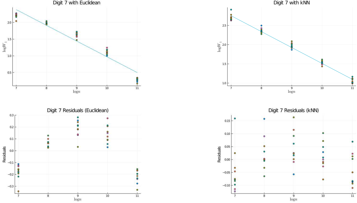
Figure 1: Two log-log plots of comparing how W_1(P_n, P'_n) decays to how W_1^M(P_n, P'_n) decays as n gets larger, as well as the residuals from a linear fit. The data are images of the digit 7 from MNIST with Wasserstein distances computed with the Sinkhorn algorithm (Cuturi, 2013). The manifold distances are approximated by a k -NN graph, as described in Section 3.
