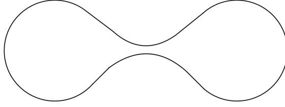
Figure 2: Curve in \mathbb{R}^2 where \tau \ll \iota .
