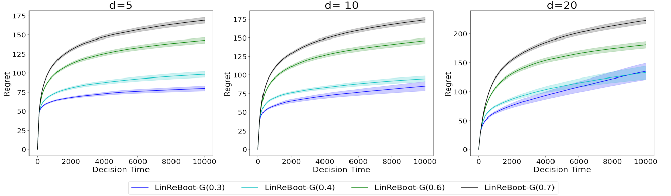
Figure 3: Second Step Tuning for LinReBoot-G under Stochastic Linear Bandit. The x axis is round t and y axis is cumulative regret. The candidate set for \sigma_\omega is \{0.3, 0.4, 0.6, 0.7\} and these three plots from left to right corresponds to d = 5 , d = 10 and d = 20 respectively.
