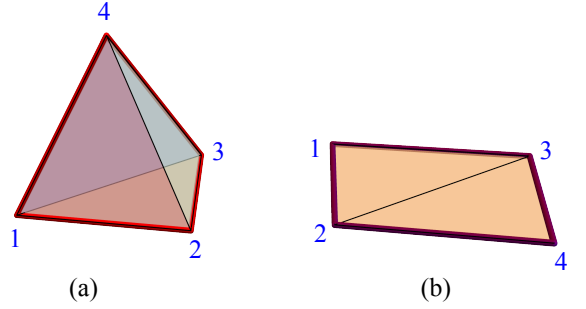
Figure 3: (a) Regular tetrahedron twists to (b) doubly-covered parallelogram.
