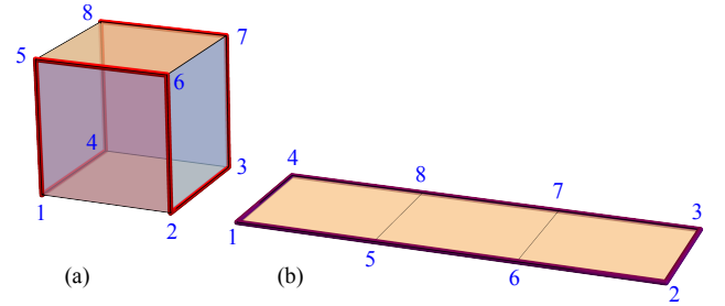
Figure 4: (a) Q = 15623784 . (b) 3 \times 1 doubly-covered rectangle.
