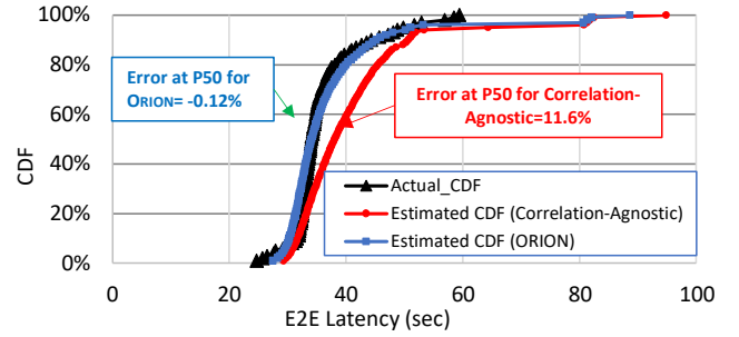
Figure 17: ORION’s estimated latency CDF vs Actual CDF for Video Analytics application deployed in Azure Functions. Ignoring in-parallel correlation leads to higher errors for the Correlation-Agnostic baseline.
