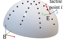
Figure 1: Tactile Sensor Representation.
