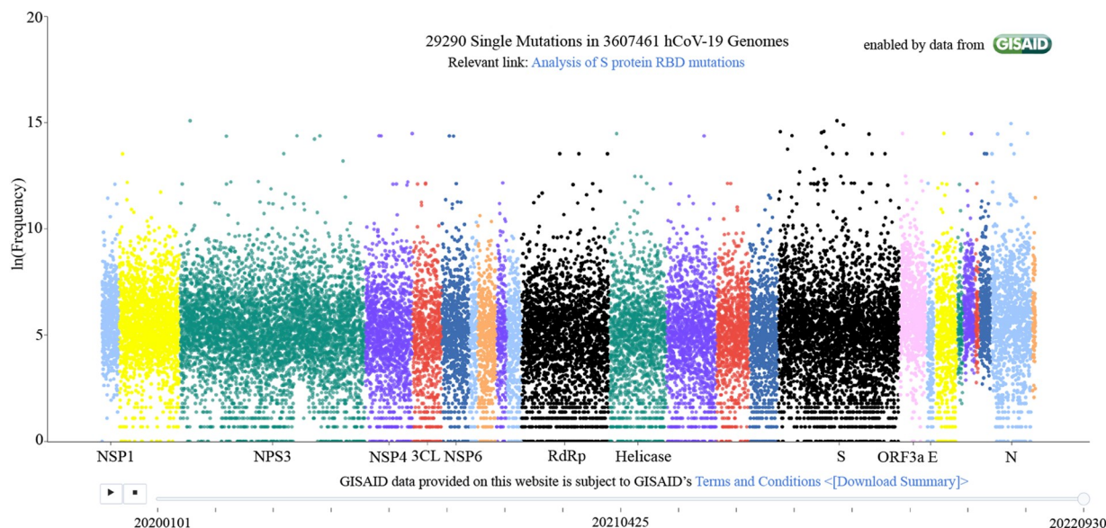
Figure 2. Illustration of unique mutations on SARS-CoV-2 genomes extracted from patients. Each dot represents a unique mutation. The x-axis is the gene position of a mutation, and the y-axis represents its observed frequency in the natural logarithmic scale.
