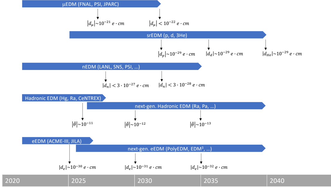
FIG. 6. Timelines for the major current and planned EDM searches. Their measurement goals are indicated by the black arrows, based on the current plans of the various groups. The Storage Ring proton EDM experiments highlighted in this report are labeled “srEDM.”
