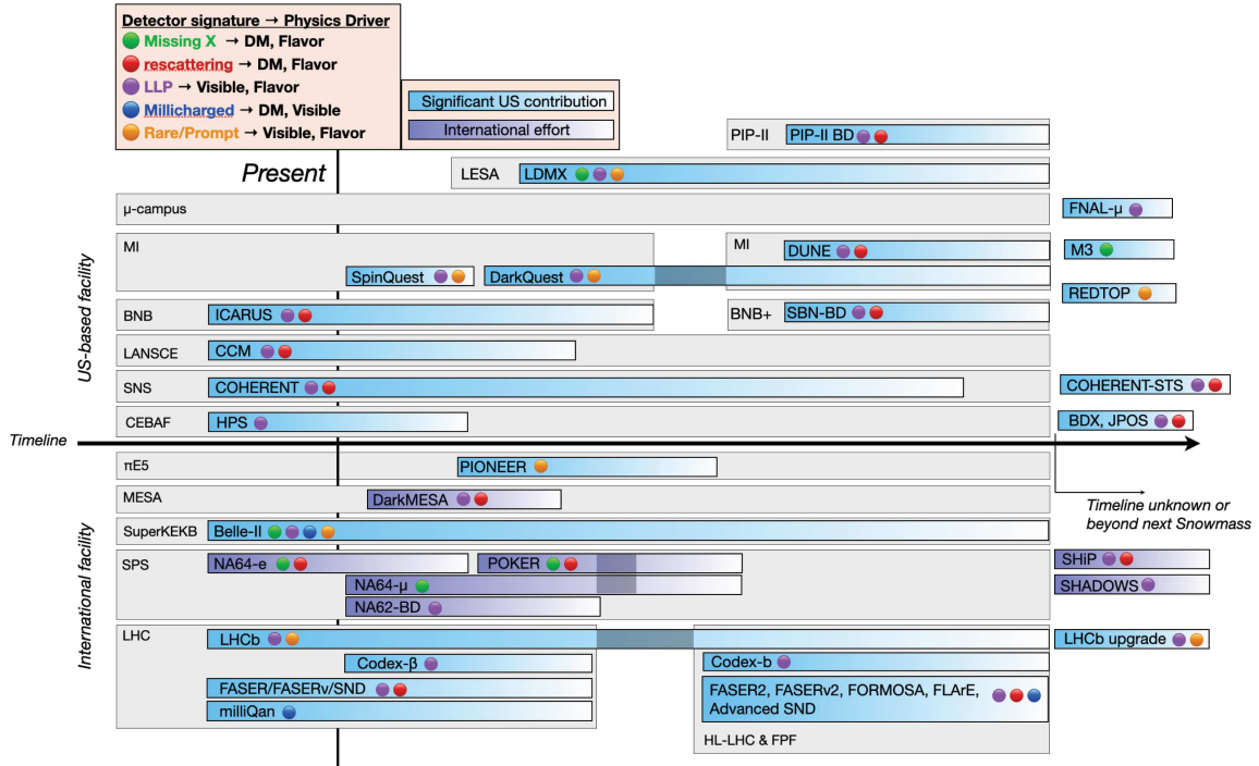
FIG. 3. Timeline for the proposed experimental program to study the dark sector at high-intensity beams and machines (from [84]).
