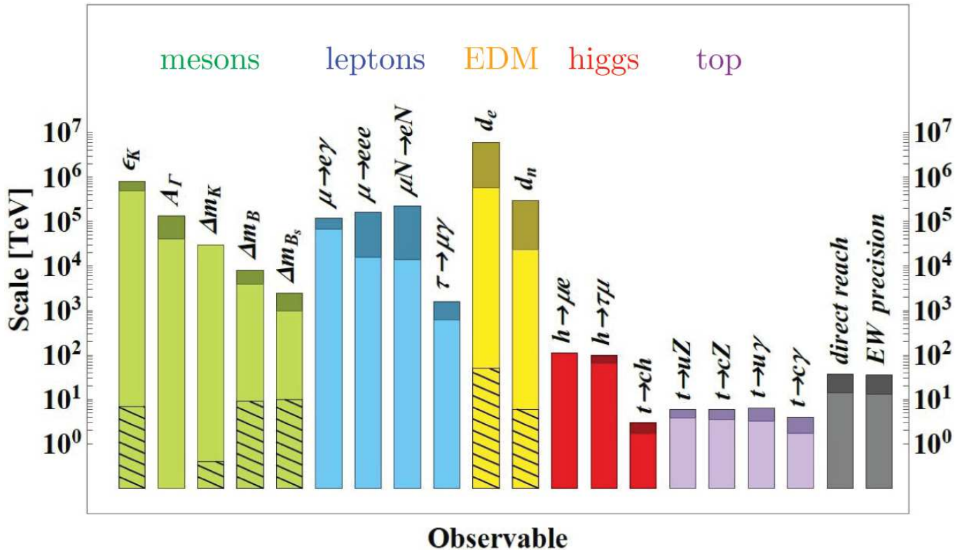
FIG. 1. Reach in new physics of present and future facilities, from generic dimension-six operators. Different probes are identified by color coding: green is for mesons, blue for leptons, yellow for EDMs, red for Higgs flavored coupling, and purple for the top quark. The grey columns illustrate the reach of direct searches and electroweak precision studies. The coupling coefficients of these operators are taken to be of \mathcal{O}(1) in the solid color columns or suppressed by MFV factors (hatch-filled surfaces). Light colors correspond to present data, and dark colors correspond to mid-term prospects in the time scale of the HL-LHC [17, 18].
