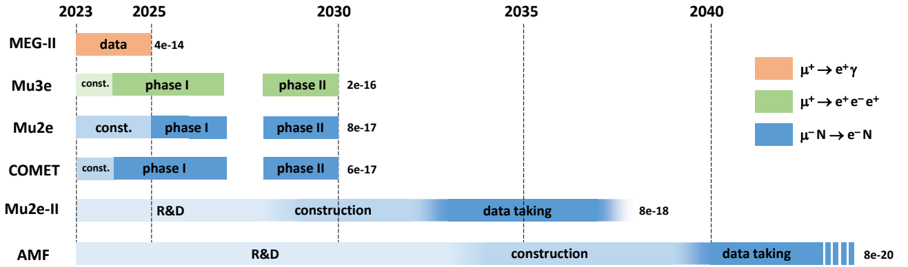
FIG. 5. Timeline for muon-based charged lepton flavor violation experiments discussed in this report. Approximate expected dates are shown. The number to the right of the timeline is the expected final 90% CL.
