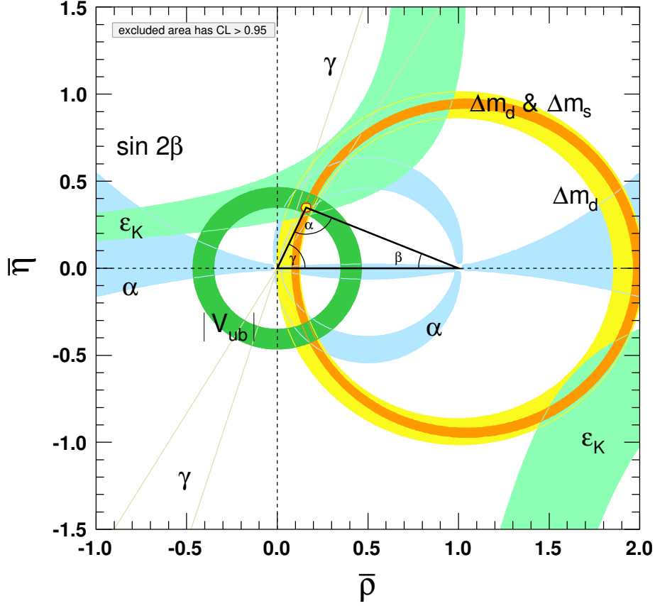
FIG. 8. Various indirect studies of New Physics can be combined to provide constraints on both SM and BSM parameters. An example is studies of the CKM unitarity triangle [35], which requires precise knowledge of nonperturbative parameters.
