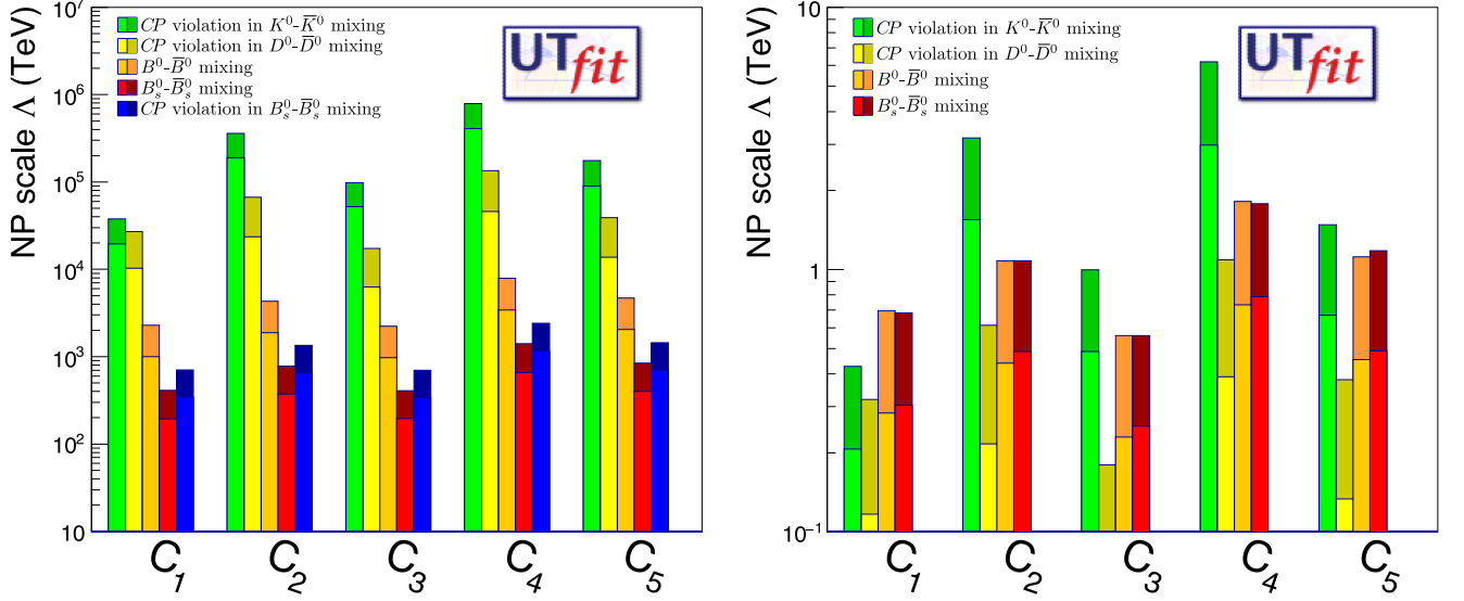
FIG. 7. Present (lighter) and future (darker) lower bounds at 95% confidence level on the NP scale \Lambda from \Delta F = 2 transitions [104, 105]. The Wilson coefficients C_i = F_i L_i / \Lambda^2 ( i = 1, \dots, 5 ) are the coupling of the NP dimension-six operators governing the \Delta F = 2 transition: Q_1^{q_i q_j} = (\bar{q}_{jL} \gamma_\mu q_{iL}) (\bar{q}_{jL} \gamma^\mu q_{iL}) , Q_2^{q_i q_j} = (\bar{q}_{jR} q_{iL}) (\bar{q}_{jR} q_{iL}) , Q_3^{q_i q_j} = (\bar{q}_{jR} q_{iL}) (\bar{q}_{jR} q_{iL}) , Q_4^{q_i q_j} = (\bar{q}_{jR} q_{iL}) (\bar{q}_{jL} q_{iR}) (with \alpha and \beta being color indices). On the left, NP is assumed to have arbitrary flavor structure ( F_i = 1 ) and to be strongly coupled with no loop suppression ( L_i = 1 ); on the right, NP is assumed to have minimal-flavor-violation couplings ( F_i = V_{CKM} ) and to enter at one loop with weak coupling ( L_i = \alpha_2^2 , with \alpha_2^2 being the weak structure constant). The future bounds are based on expected sensitivities at Belle II ( 50 \text{ ab}^{-1} ), BESIII, LHCb Upgrade II ( 300 \text{ fb}^{-1} ), and ATLAS/CMS ( 3 \text{ ab}^{-1} ), and on improved theory inputs (from [31]).
