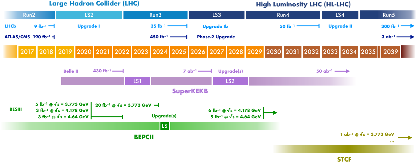
FIG. 2. Timeline for the proposed experimental program in heavy flavor physics.
