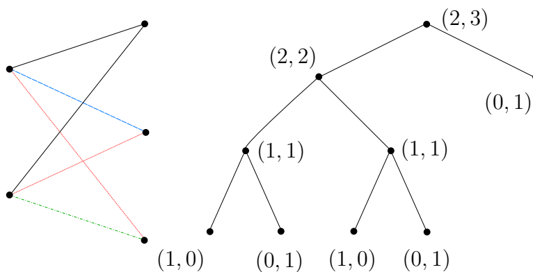
Figure 2: A JL-coloring of K_{2,3} and its associated JL-tree.
