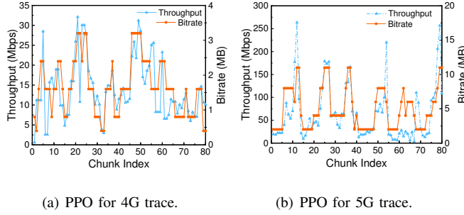
Fig. 11. A case of bandwidth and chunk bitrate by different network traces.
