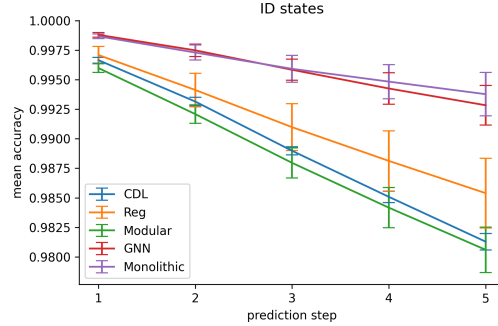
Figure 21. Multi-step prediction performance for the physical environment.
