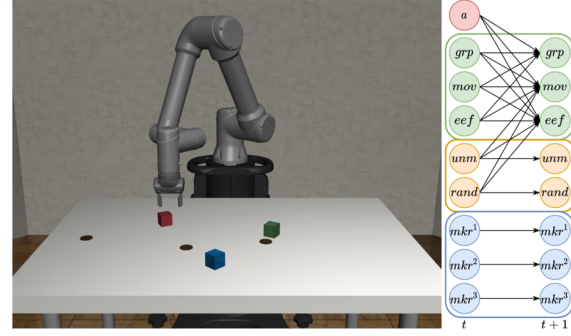
Figure 5. (Left) the manipulation environment. (Right) the learned causal graph in the object level which recovers the ground truth relationship between the state variables and the action.
