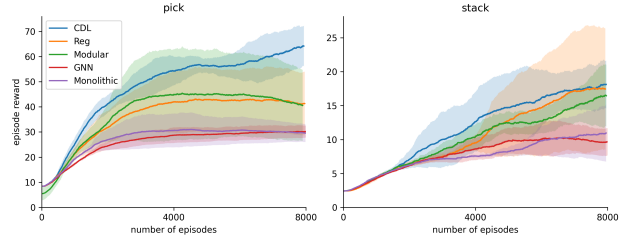
Figure 7. Training curves for two downstream tasks.
