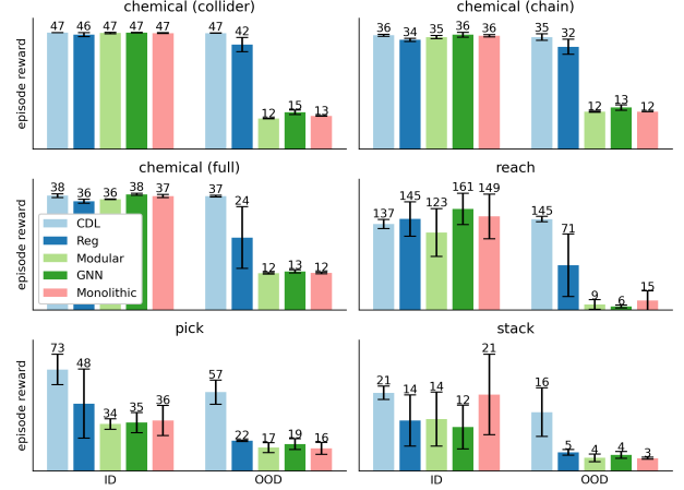
Figure 8. Episode reward of learned policies on ID and OOD states. movable object.
