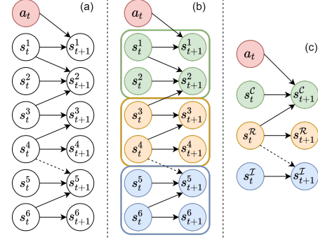
Figure 2. (a) an example causal dynamics model. (b) state variables can be split into three types: controllable (green), action-relevant (orange), and action-irrelevant (blue). The dashed arrow represents whether it exists does not affect s_t^5 to be action-irrelevant. (c) the causal graph can be split into three subgraphs, one for each type of state variable.
