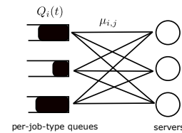
Figure 1: A Multi-Server System With Three Servers and Three Types of Jobs.
