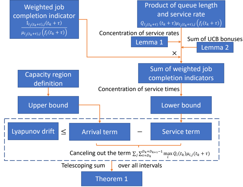
Figure 4: The proof roadmap of Theorem 1.
