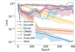
(b) Ground energy search
