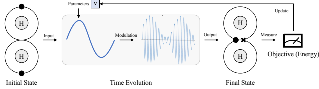
(a) Analog-ansatz-based VQE for the H_2 system
