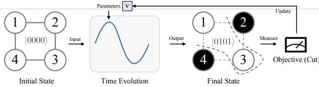
(c) Analog-ansatz-based QAOA for a MaxCut problem
