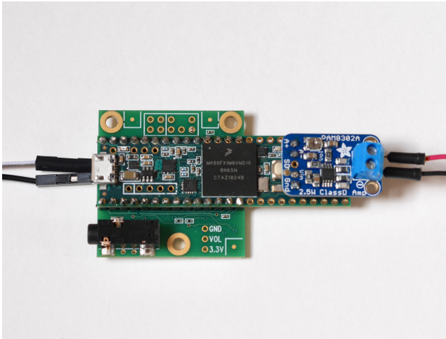
Figure 3: The Teensy 3.6, Audio breakout board, and audio amplifier assembly.
