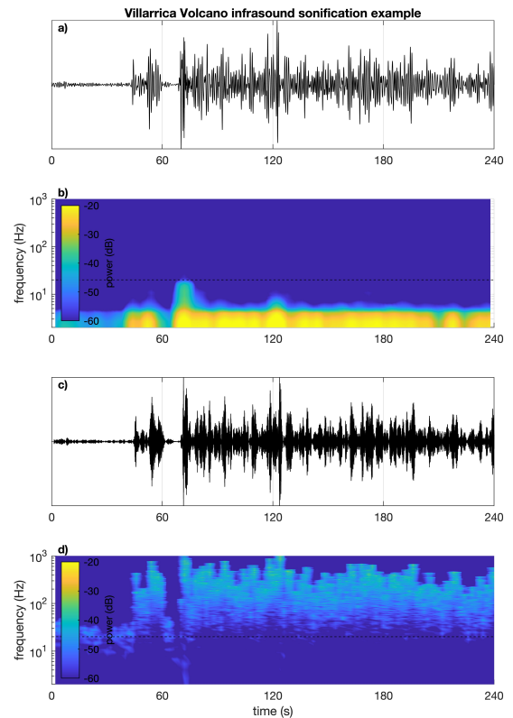
Figure 2: a) Infrasonic collected at the Volcán Villarrica crater rim. b) Spectrogram calculated with 4 s windows and 2 s overlap. c) Processed infrasound using carrier frequency of 50 Hz and an index of modulation of 20. d) Corresponding spectrogram for panel c with 4 s windows and 2 s overlap. Spectrogram power is given in dB/Hz.
