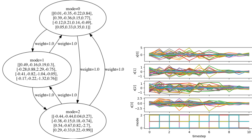
Figure 7: Microbenchmark (Left) with n = 4, m = 3 and sample trajectories (Right).
