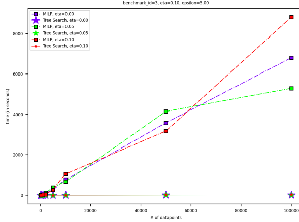
Figure 3: Plot showing how the two approaches - 1) MILP (dashed lines) and 2) proposed approach (solid lines) scale in terms of times taken to solve the system identification problem as the number of data points increases. The plot reports time taken by both approaches for dataset size N = 10 to N = 100000 from Benchmark #3 ( n = 5 , m = 8 ).
