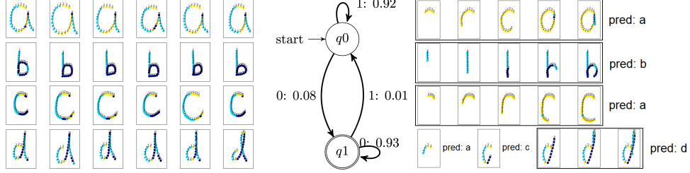
Figure 4: Left: Handwriting samples with identified modes shown in different colors, Middle: JMM model for letter b and Right: predicting letters from partial observations using the JMM.
