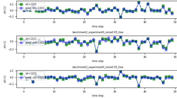
Figure 2: Plot showing the actual trajectory (in green) and the estimated trajectory (in blue) by the tree search algorithm for benchmark #2 and N = 50 .
