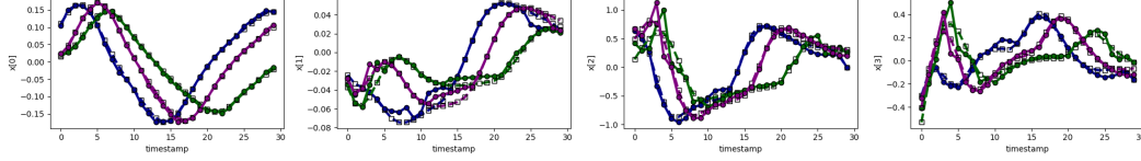
Figure 9: 3 trajectories of the Cartpole benchmark: The dashed lines with square markers show the reference trajectories. The solid lines with triangle markers show the trajectories predicted using the dynamics identified by the proposed approach.
