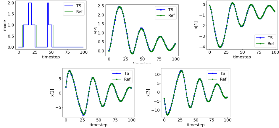
Figure 6: Data from the Acrobot system plotted against those of the identified model.
