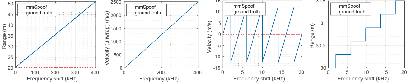
(a) Distance estimated on radar (b) Unwrapped velocity estimated on radar (c) Estimated velocity on the radar (Subset) (d) Estimated distance on the radar (Subset)
