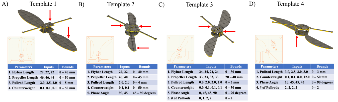
Fig. 5. Flybar design templates: A) Template 1. The unique features of this design is the rectangular flybar and propeller plates, as well as the lack of a leading edge on the propellers. B) Template 2. The unique features of the design are the rounding of the flybar and propeller plates, leading edges on the propellers, and manual puzzle piece like attachments for the flybars. C) Template 3. The unique features of the design were the changed axis of rotation for the connecting rod between and a manual attachment for the flybar that fit into cutouts of the top layer of the laminate. D) Template 4. The unique feature of the design is the altered connecting pullrod to allow for 45 degree alpha angles between the two plates that properly feathers the rotor.
