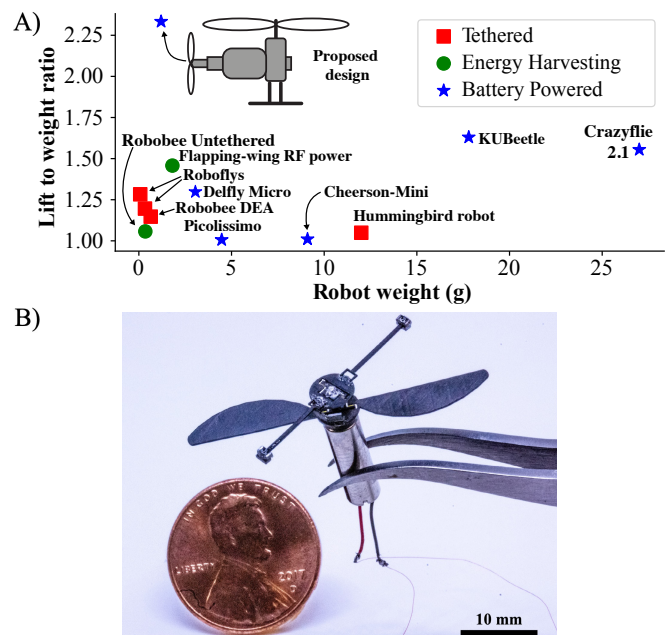
Fig. 1. A) Plot of lift to weight ratio, including mass of battery and power harvesting payload, for small aerial robots: Roboflys [2, 3], Robobee DEA [4], Robobee Untethered [5], Piccolissimo [6], Cheerson-Mini [7], Crazyflie 2.1 [8], Flapping-wing RF power [9], KUBeetle [10], Hummingbird robot [11], and DelFly Micro [12]. B) Flybar-rotor mechanism attached to a motor. Flybar tilting mechanically changes the rotor angle of attack.
