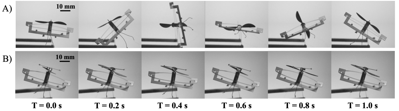
Fig. 9. A) Video frames from 1 s of a 2D stability test with no flybar showing a motor with near zero damping. B) Video frames from 1 s of a 2D stability test with our template 4 flybar achieving a damping ratio of ( \zeta = 0.528 ). Small amounts of gyroscopic precession are seen about the center axis.
