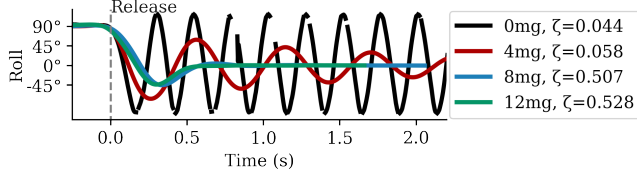
Fig. 7. Counterweight vs 1D Damping: Roll angle response of flybar template 4 with different counterweights exhibiting increased damping with increased counterweight. MoCap cameras occasionally miss data points.
