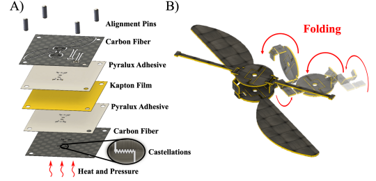
Fig. 3. A) Pin aligned laminate showing the 5 layer stack and castellated hinge joints with micrometer-size features. B) Arrows indicate the folds used to assemble the flat laminate template 4 design into a 3D flybar.
