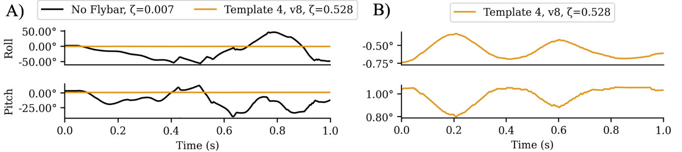
Fig. 10. Motion capture data from the same 2D test shown above. A) Pitch and roll angle response comparison of a flybar template 4 prototype and a rotor without a flybar. B) Zoomed-in pitch and roll angle response of a flybar template 4 prototype.
