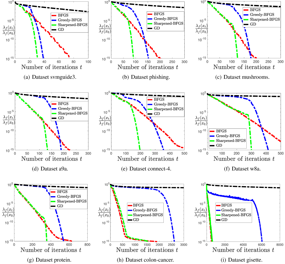
Figure 2. Comparison of BFGS, Greedy-BFGS, Sharpened-BFGS and gradient descent (GD) on different datasets.
