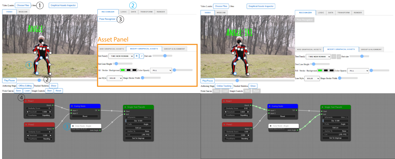
Figure 4: Overview of how users could author and test a pose effect using PoseVEC. Here the user is creating an effect that could dynamically render the angle value of the right knee on the video. Left: The PoseVEC interface in offline editing mode. Right: The PoseVEC interface in online tracking mode. In offline editing mode, we show the steps for creating a pose recognizer by scrubbing the video (black numbered annotations) and steps for creating a pose-related data node through joint selection on video canvas (blue numbered annotations). In online tracking mode, users can see the pose effect happens on the video canvas and observe the data flow in the pose program.
