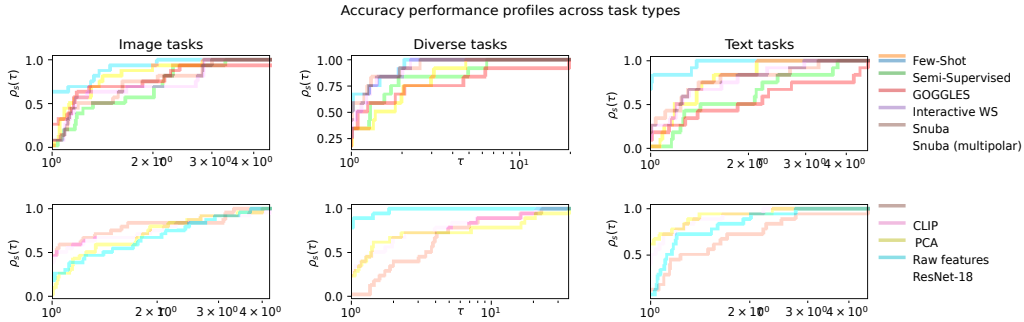
Figure 2: For image tasks (left)—MNIST, CIFAR-10, Spherical MNIST, Permuted MNIST—few-shot learning and CLIP both dominate. For diverse tasks (center)—ECG, Navier-Stokes, Ember—Snuba closes the gap with few-shot learning and CLIP underperforms or is non-applicable. For text tasks (right)—YouTube, Yelp, IMDb—few-shot learning and raw features (i.e., BERT embeddings), while the CLIP text encoder alone underperforms or faces compatibility issues with IWS.
